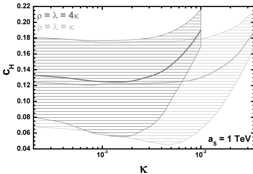
Figure 4: The parameter values (\kappa, c_H) allowed by (3.1), (3.5) and (3.10) in the nmSUGRA scenario, for \rho = \lambda = \kappa (light grey hatched area) and \rho = \lambda = 4\kappa (grey hatched area). The grey (light grey) line has been obtained by fixing n_s to its central value given in (3.10), for \rho = \lambda = 4\kappa ( \rho = \lambda = \kappa ).
