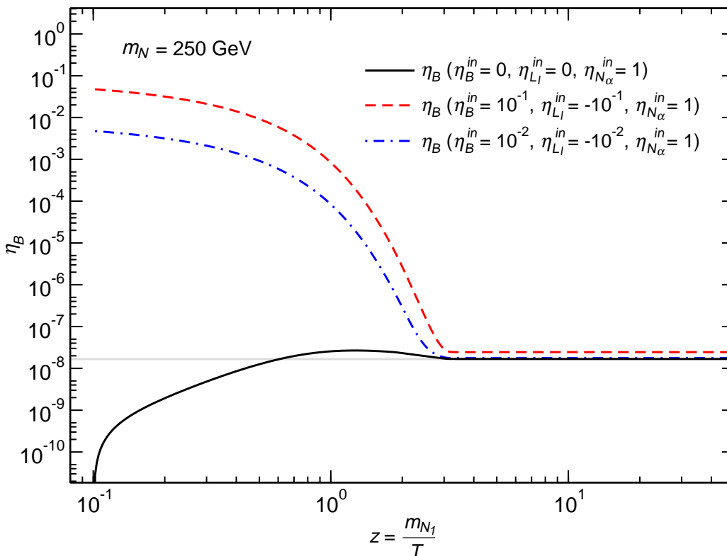
Figure 10: Numerical estimates of the BAU for a scenario with m_N = 250 GeV and for different initial lepton- and baryon-number abundances, \eta_{L_l}^{\text{in}} and \eta_B^{\text{in}} , assuming an initial thermal distribution for the heavy Majorana neutrinos, i.e. \eta_{N_{1,2,3}}^{\text{in}} = 1 . The horizontal grey line shows the BAU needed to agree with today’s observed value.
